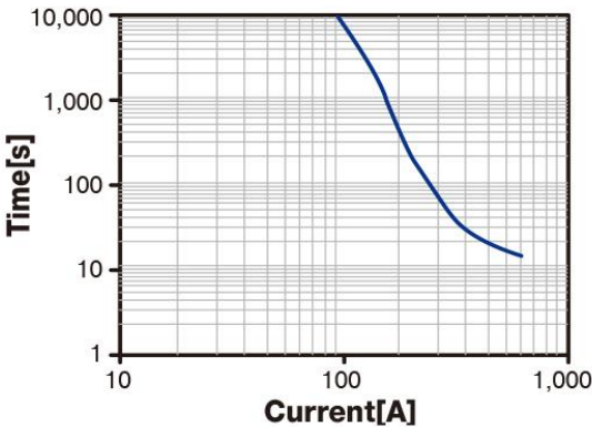
Current Distribution(35mm 2 at 85°C)
