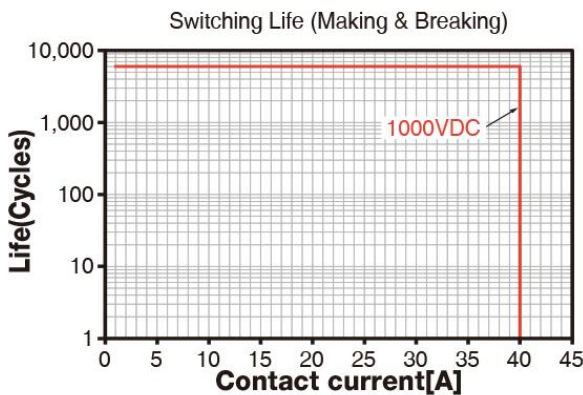
Switching/ Cut-off Curve
