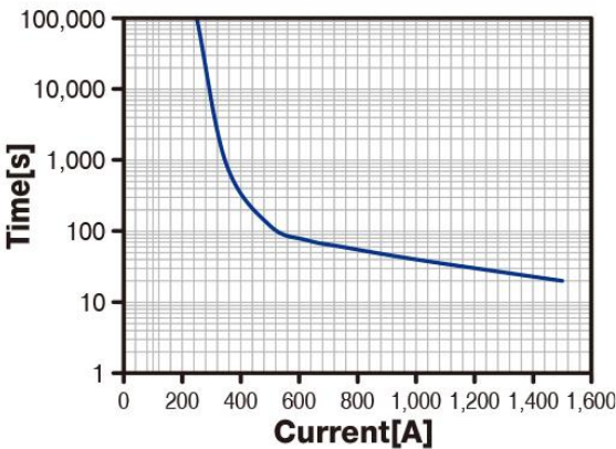
Current Distribution(120mm 2 at 85°C)
