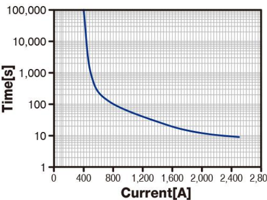
Current Distribution(120mm 2 at 85°C)
