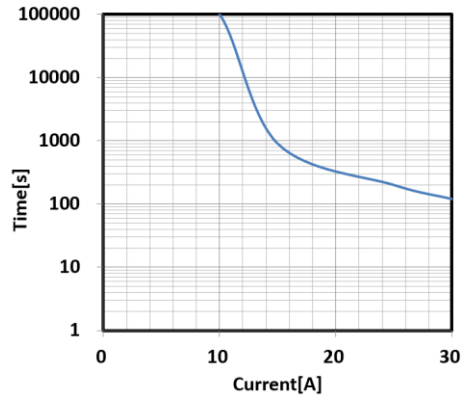
Current Distribution (2mm 2 at 85°C)
